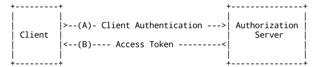
Figure 6: Client Credentials Flow
